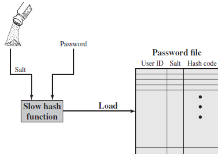
(a) Loading a new password
